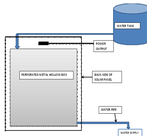
Fig.2.4 Working Line Diagram Of Project
