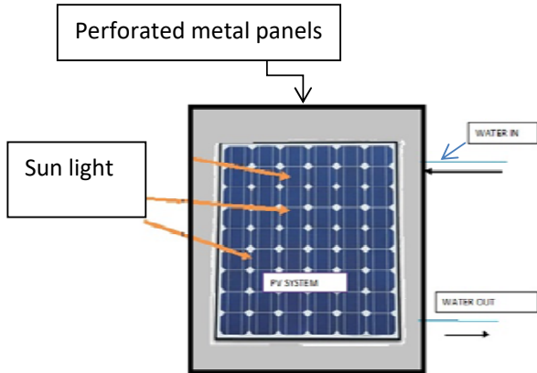
Fig .2.5. ARRANGEMENT OF SOLAR PANEL, PERFORATED METAL PANEL AND NOZZLES
