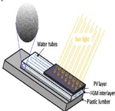
Fig.1 Schematic illustration of the hybrid solar roofing panel prototype.
