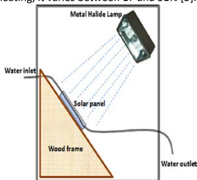
Fig. 2 Solar panel testing set-up
