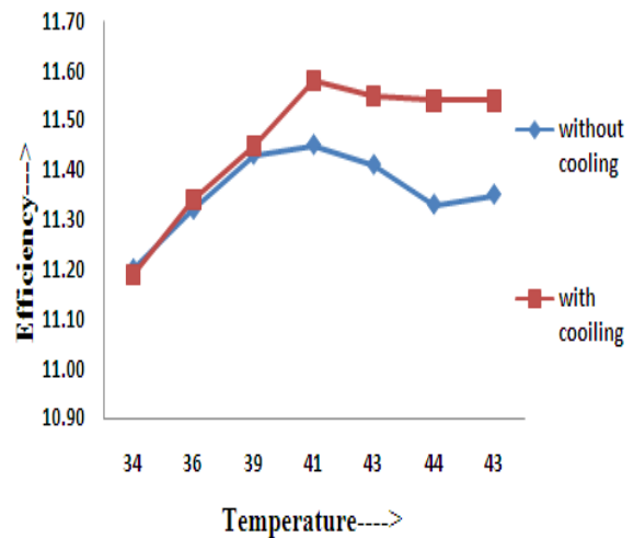
Fig. 8 Variation of Efficiency with respect to Temperature
