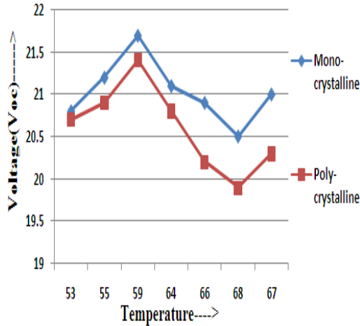
Fig.6 Variation of Voltage with respect to temperature
