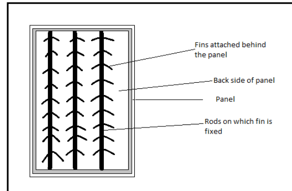
Fig. 4.2 Back view of modified panel having fins fixed on the rods
