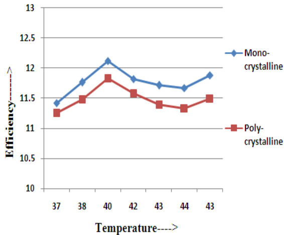
Fig. 5 Variation of Efficiency with respect to temperature.
